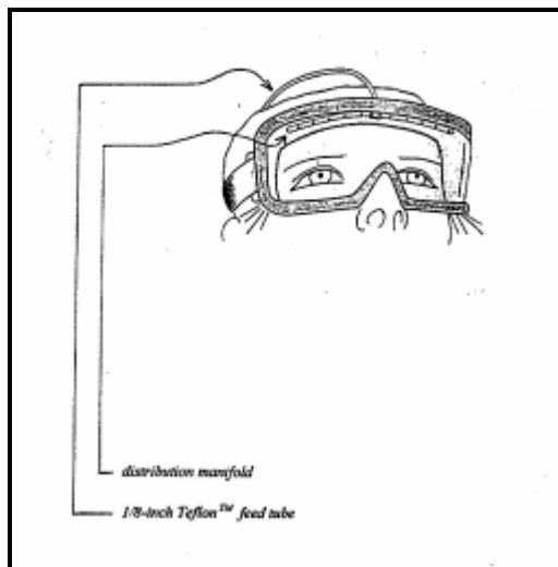
Figure 1. Diagram of Goggles Used in Methyl Isothiocyanate Experiment 66
